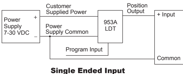
Figure 3-2: Current Sourcing
