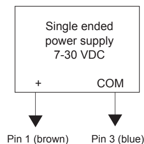
Figure 3-1: Power Supply Wiring
