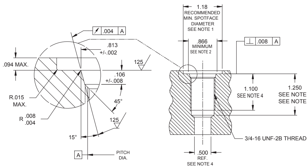
Figure 2-3: Port Detail (SAE J1926/1)
